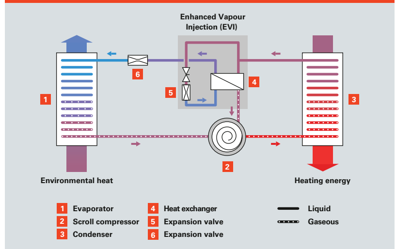
Fig. A.3.1–4 Enhanced Vapour Injection (EVI)
