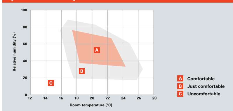
Fig. D.2.3-1 Air conditioning
