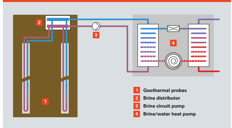
Fig. A.4.1-5 Heat source – geothermal probe
