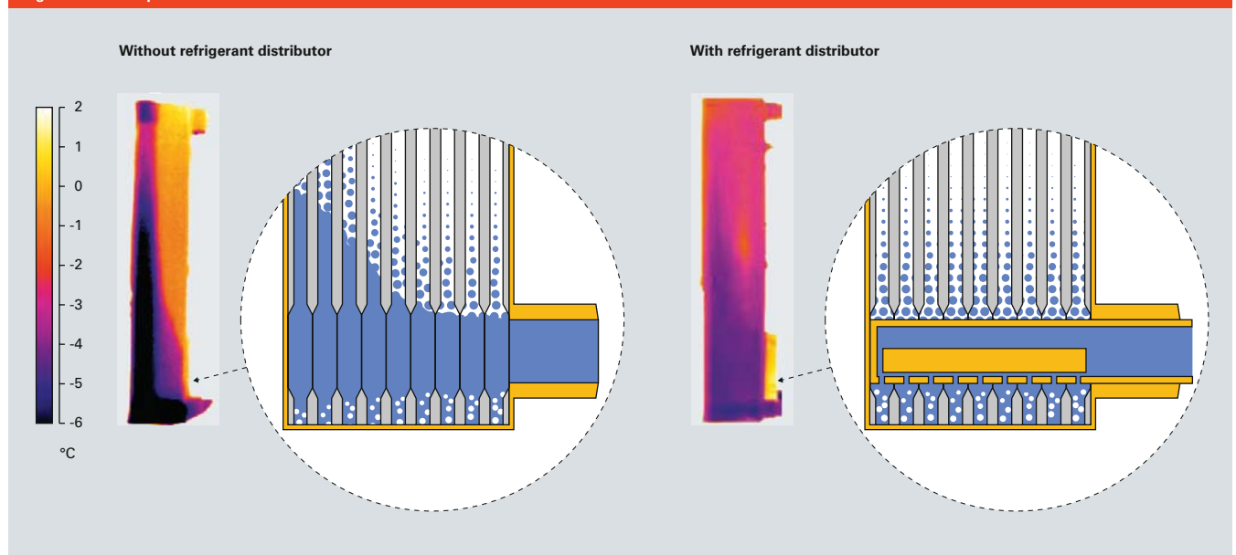
Fig. A.3.3-1 Evaporator with and without distributor
