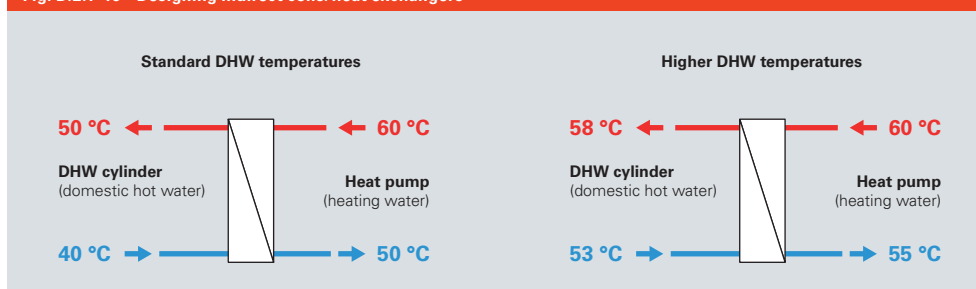
Fig. D.2.1–16 Designing indirect coils/heat exchangers
