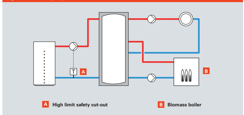
Fig. D.1.4–3 Heat pump and biomass
