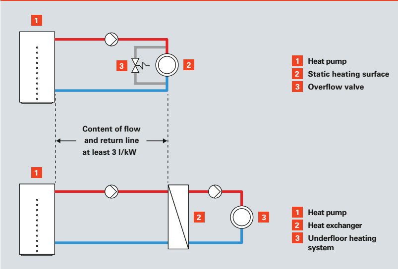
Fig. D.2.2-4 Minimum volume in the heating circuit
