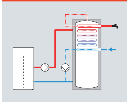
Fig. D.2.1-19 Coaxial booster heat exchanger
