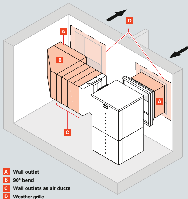
Fig. C.3.4–1 Air routing with internal installation
