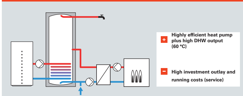
Fig. D.2.1-7 Dual mode DHW heating
