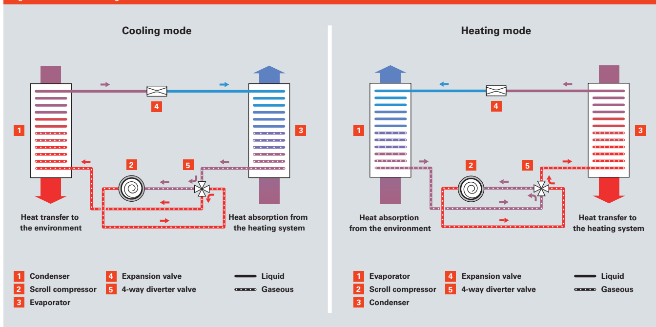
Fig. D.2.3-3 Active cooling
