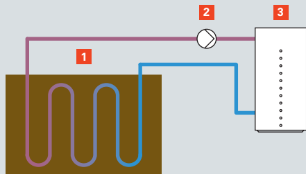
Fig. C.1.1-1 Geothermal collector and geothermal probe
