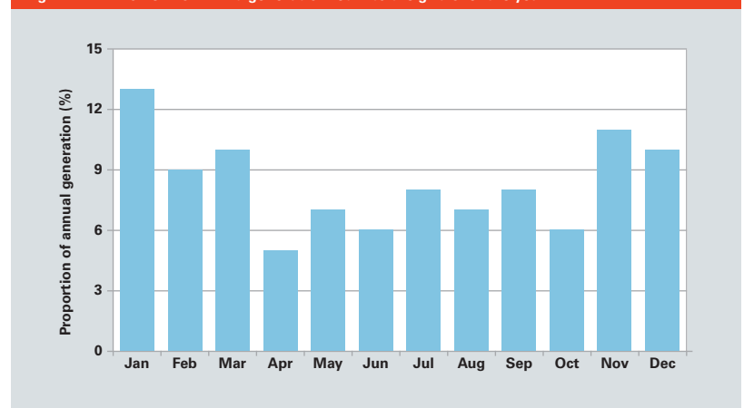
Fig. B.1.2-2 Power from wind generation fed into the grid over the year
