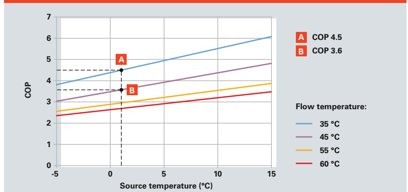
Fig. D.2.2-5 Heating circuit flow temperature and efficiency
