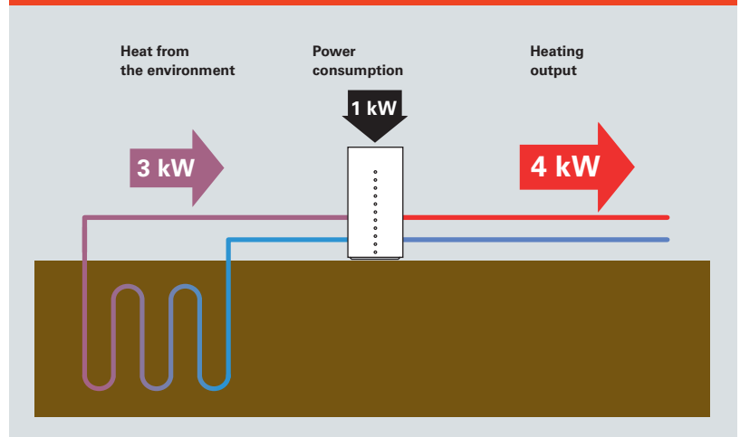
Fig. A.2.3–1 The efficiency level as coefficient of performance
