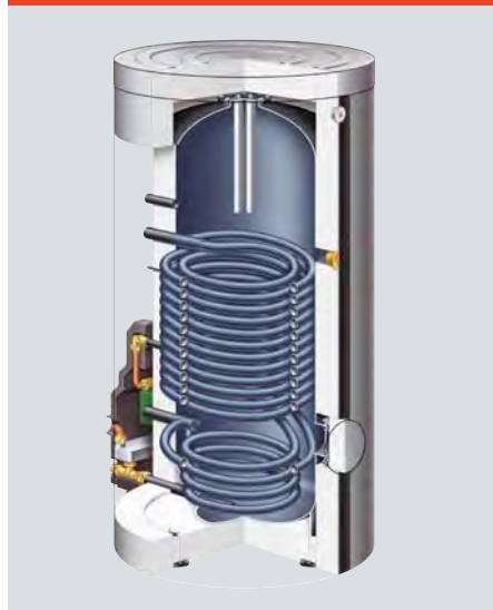
Fig. D.1.4–2 DHW cylinder
