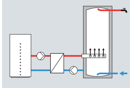
Fig. D.2.1–15 Heating lance function
