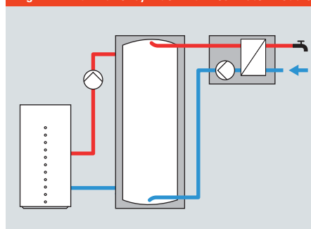
Fig. D.2.1-20 Buffer cylinder with freshwater module
