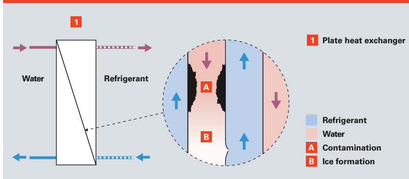
Fig. C.2.1-1 Plate heat exchanger at risk
