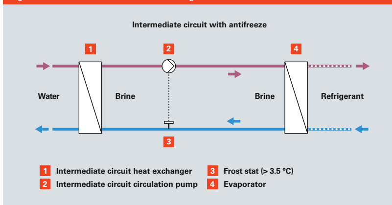
Fig. C.2.1-2 Intermediate circuit heat exchanger
