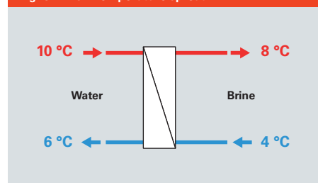
Fig. C.2.1-3 Temperature spread
