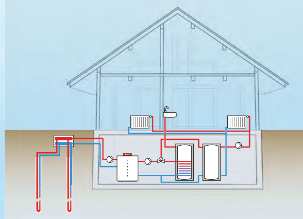
Ground source (probe)
