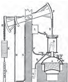
Fig. A.1-1 Newcomen steam engine
