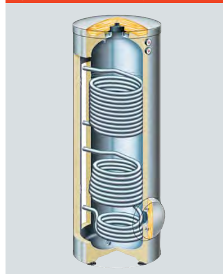
Vitocell 300-B DHW cylinder
