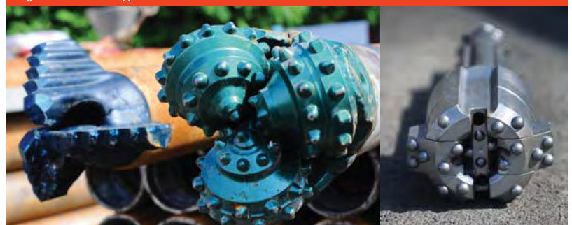
Fig. A.4.1-7 Drill types
