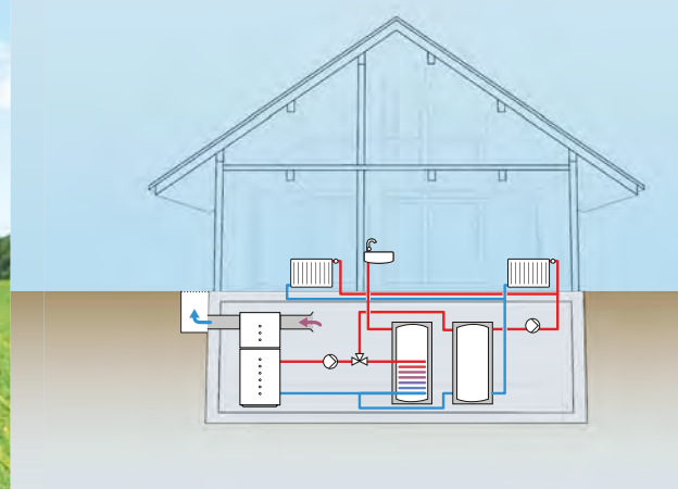
Air source
