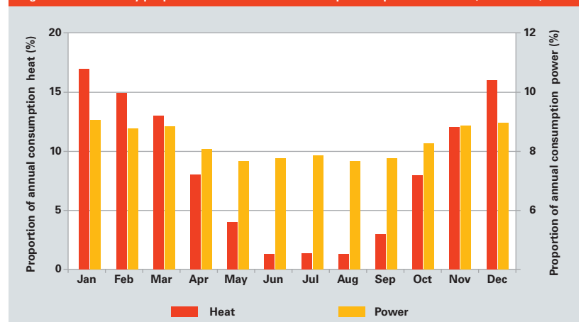
Fig. B.1.2-1 Monthly proportions of the annual consumption of power and heat (EFH sector)
