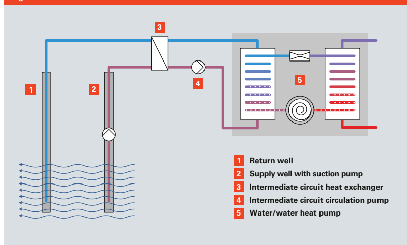
Fig. A.4.2-1 Heat source water with intermediate circuit
