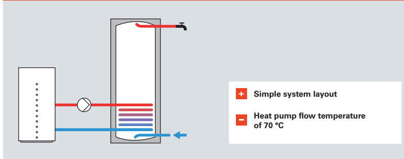
Fig. D.2.1-5 Mono mode DHW heating
