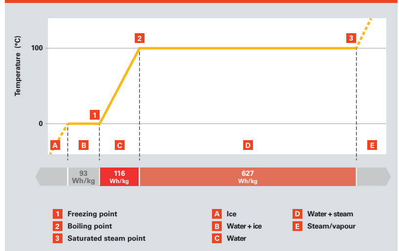
Fig. A.2.1–1 Energy content of steam
