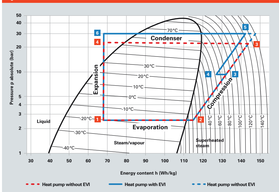
Fig. A.3.1–5 EVI effect
