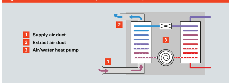
Fig. A.4.3-1 Heat source – outdoor air (internal installation)
