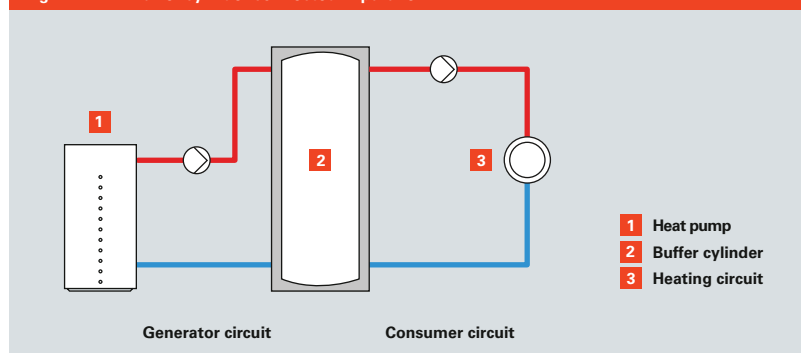
Fig. D.2.2-1 Buffer cylinder connected in parallel
