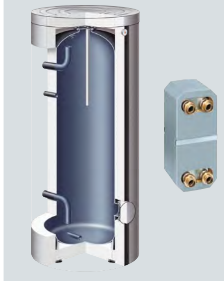
Fig. D.2.1–14 Primary store with heating lance
