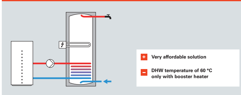
Fig. D.2.1-6 Mono energetic DHW heating
