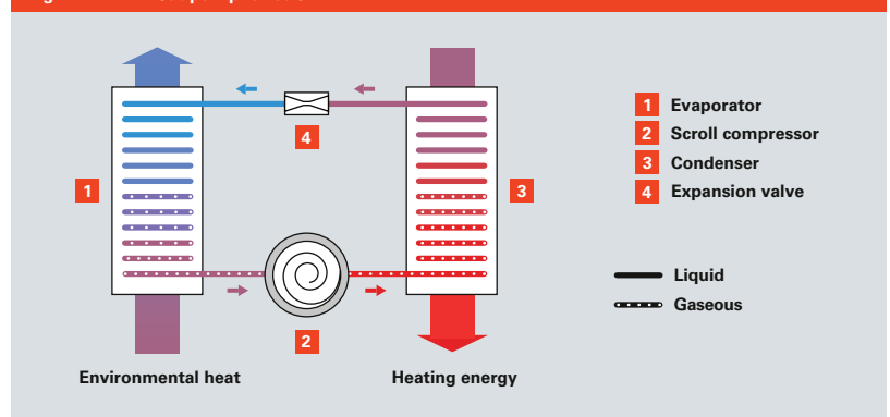
Fig. A.2.2–1 Heat pump function
