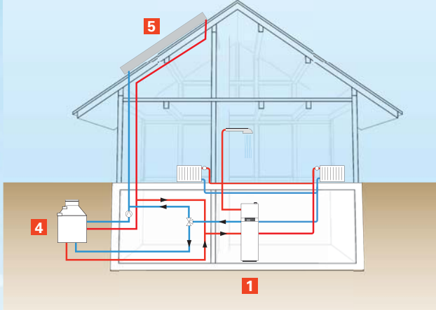
Heat from the ground, the air and the sun (ice store)
