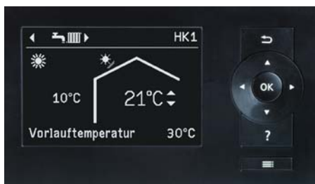
Weather-compensated Vitotronic 200 heat pump control unit (type WO1C)
