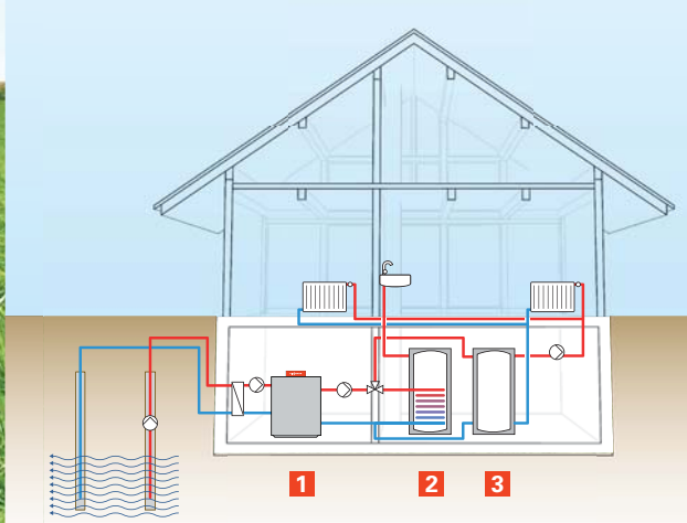
Ground source (groundwater)
