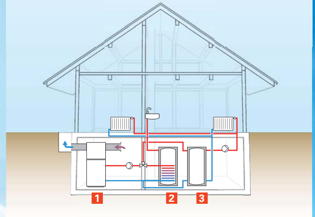
Air source
